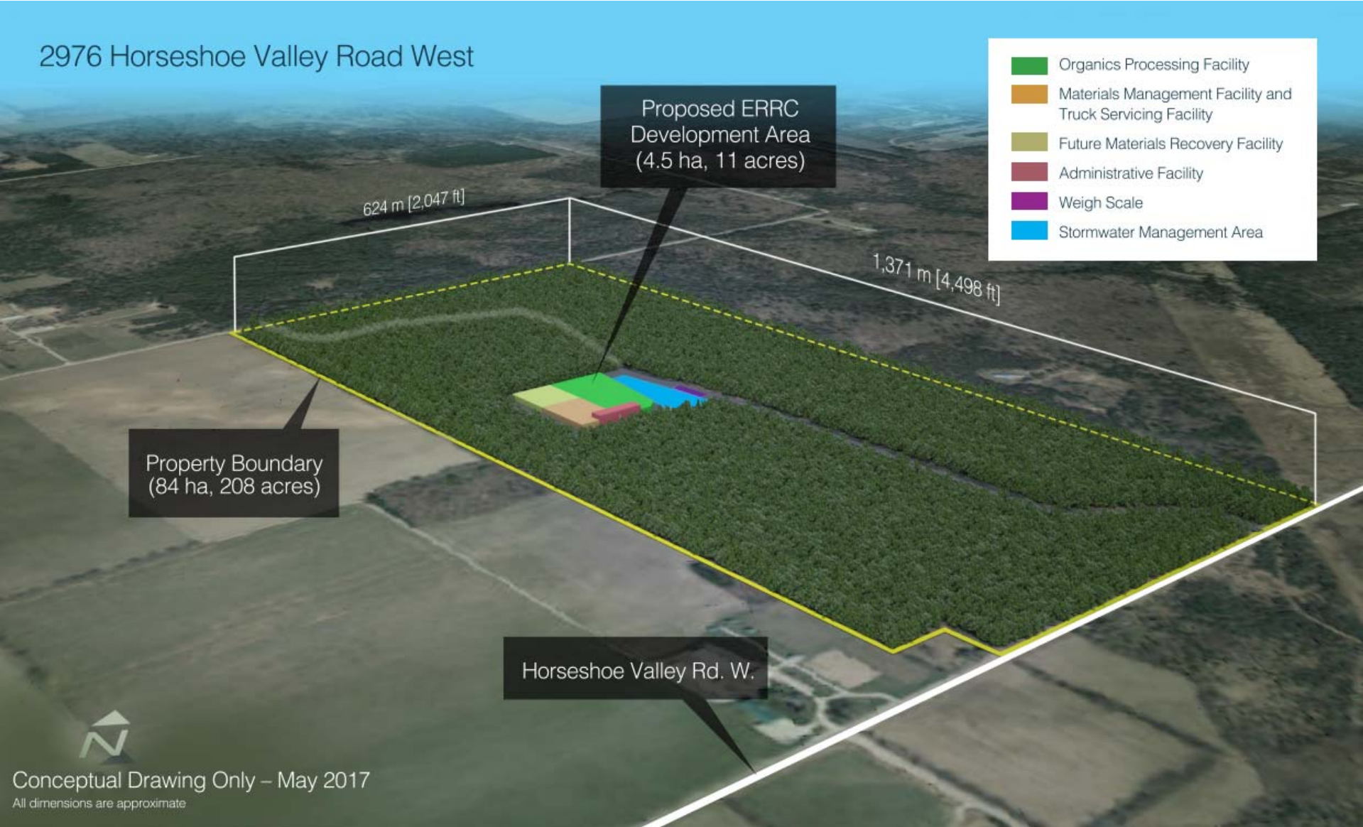
Figure 2: Conceptual Site Layout (GHD, 2017)
